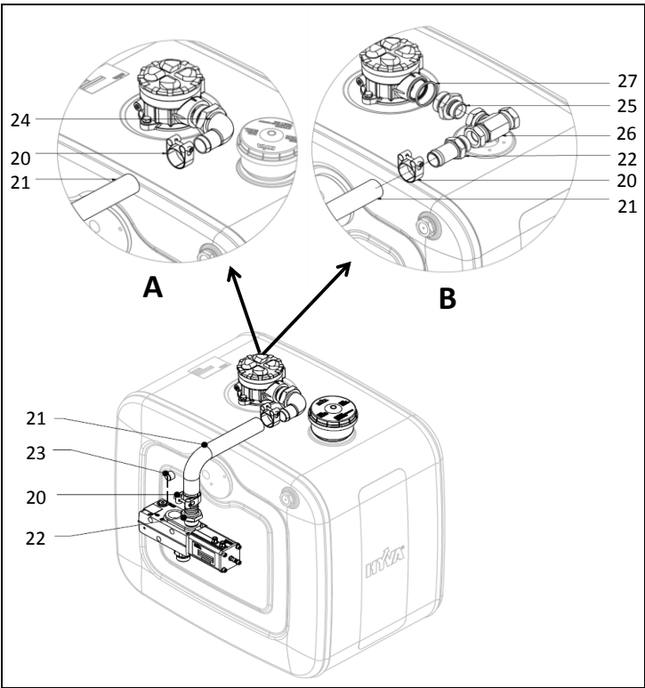
Side mounted valve
