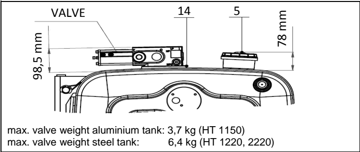
Top mounted valve
