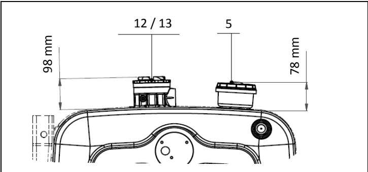
Chassis or cylinder mounted valve
