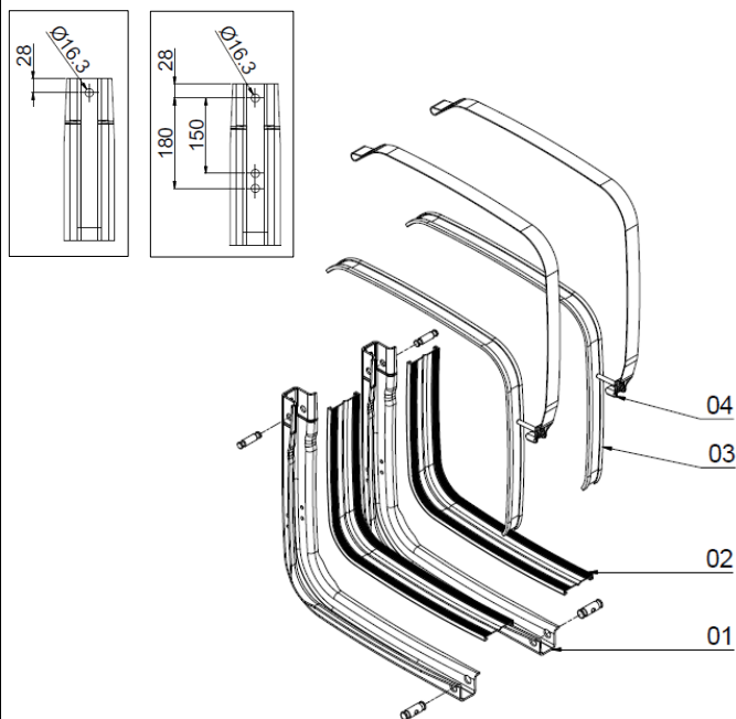
Detail support with one hole and support with three holes
